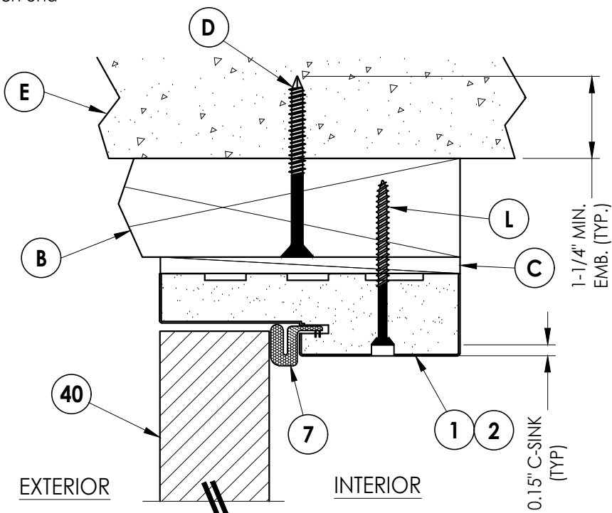
5 6 VERTICAL CROSS SECTION Outswing shown (Inswing similar)
