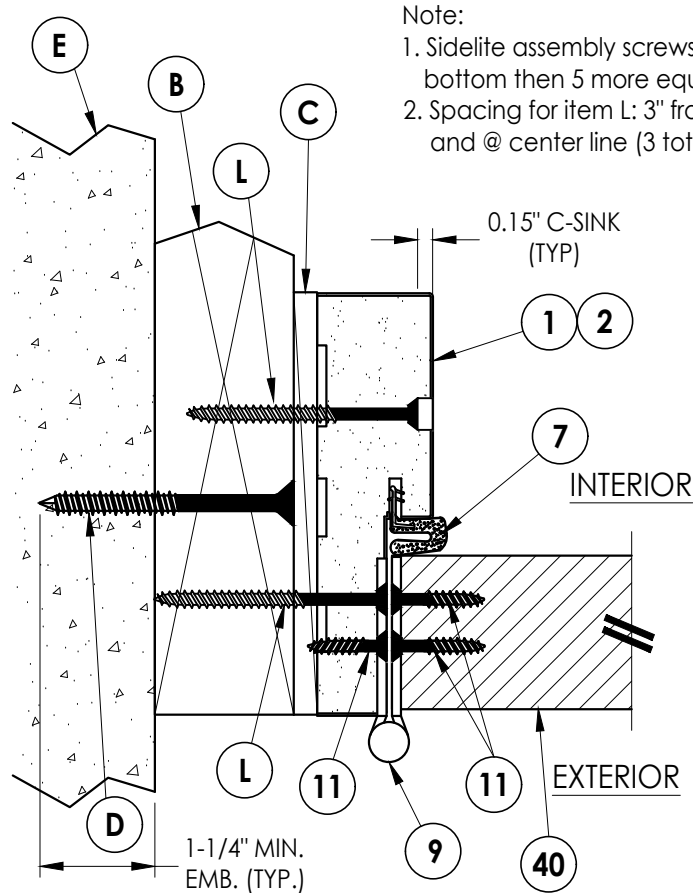
1 6 HORIZONTAL CROSS SECTION Outswing shown - Inswing also approved
