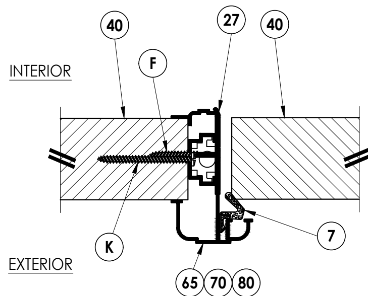
3 6 HORIZONTAL CROSS SECTION Outswing shown - Inswing also approved
