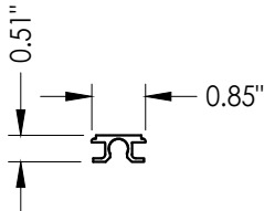
82 83 FLUSHBOLT RETAINER Top / bottom Aluminum 6063-T5
