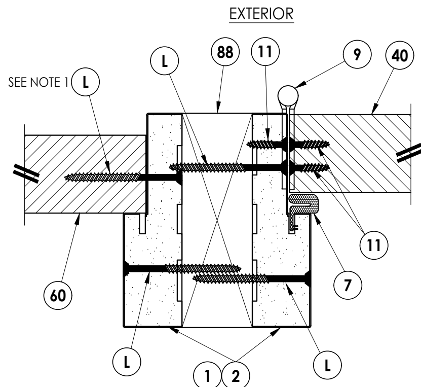
2 6 HORIZONTAL CROSS SECTION Outswing shown - Inswing also approved Shown with 1X reinforcement
