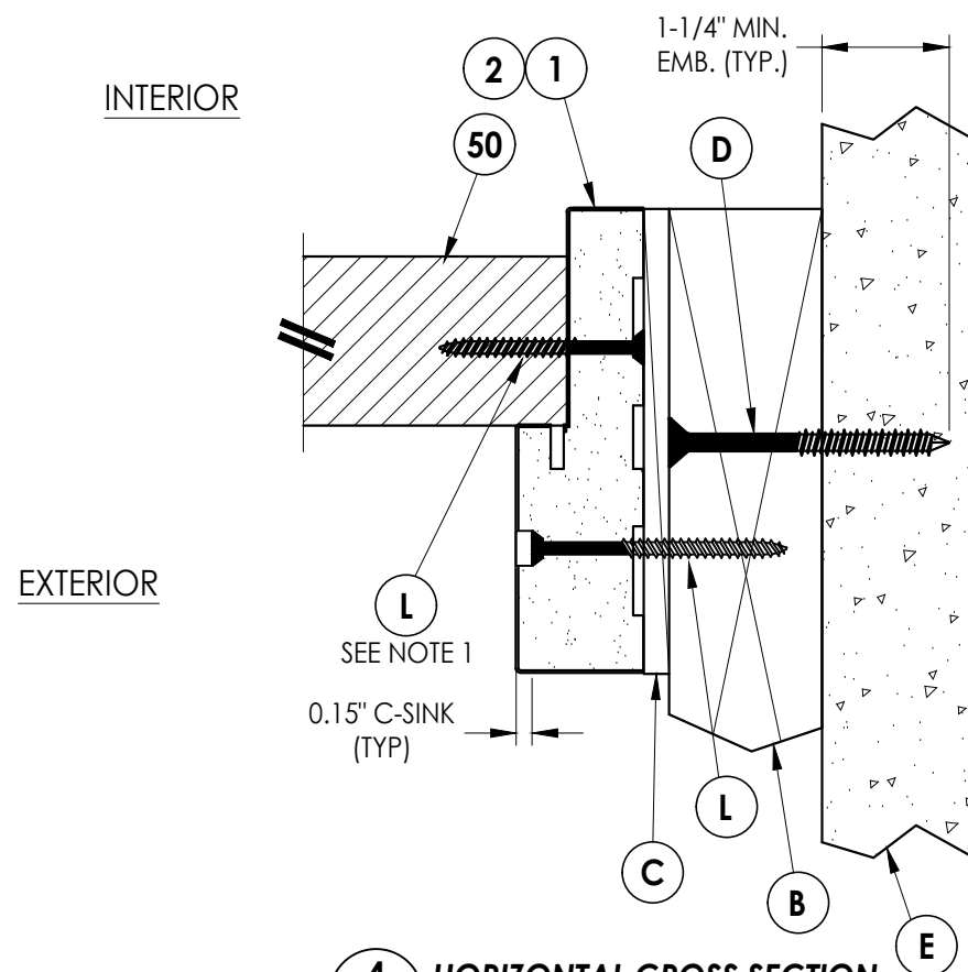
4 6 HORIZONTAL CROSS SECTION Outswing shown (Inswing similar)
